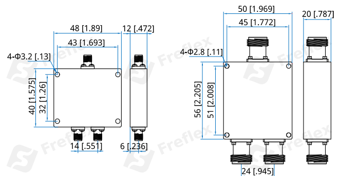
Outline A
