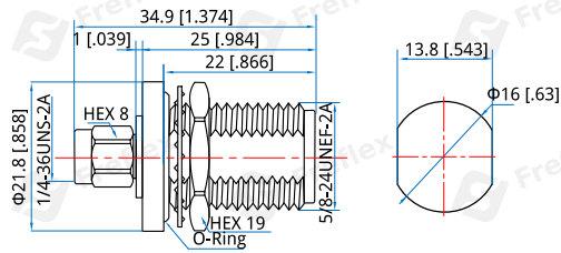
Outline I
