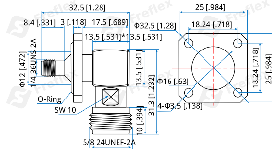
Outline J
