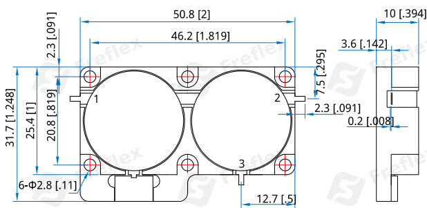
Outline A
