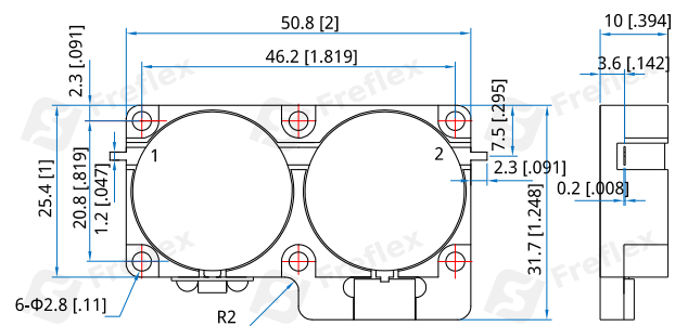
Outline B
