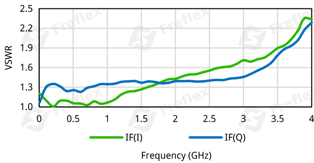
IF VSWR vs. Frequency
