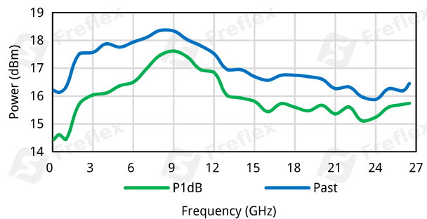
Power vs. Frequency
