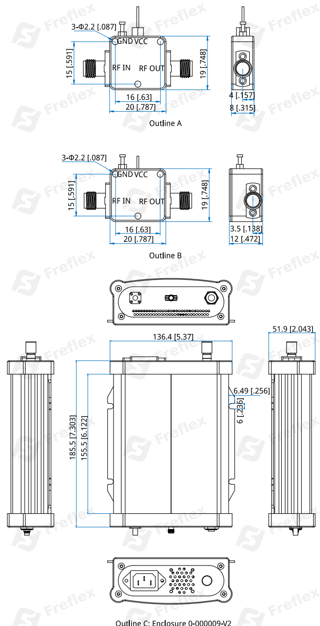
Outline C: Enclosure 0-000009-V2
