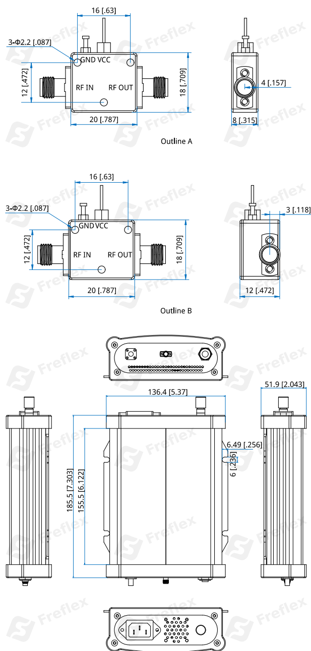
Outline C: Enclosure 0-000009-V2
