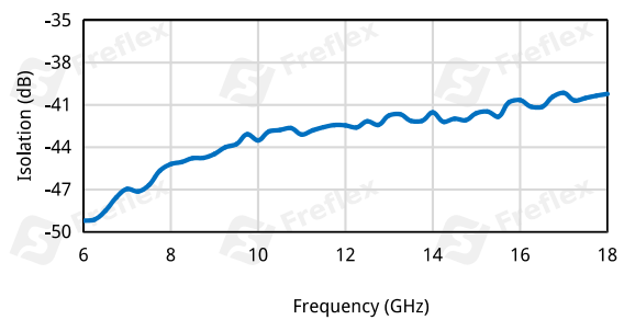
Isolation vs. Frequency
