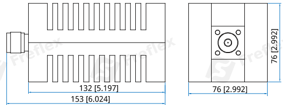
Outline A
