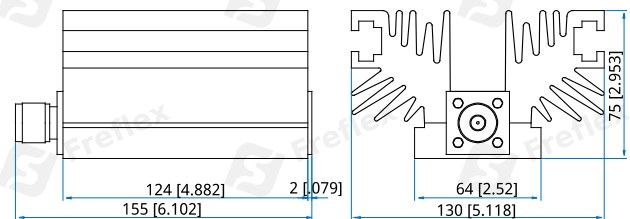
Outline B
